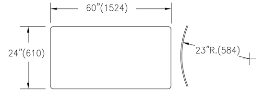
Buck Dimensions
